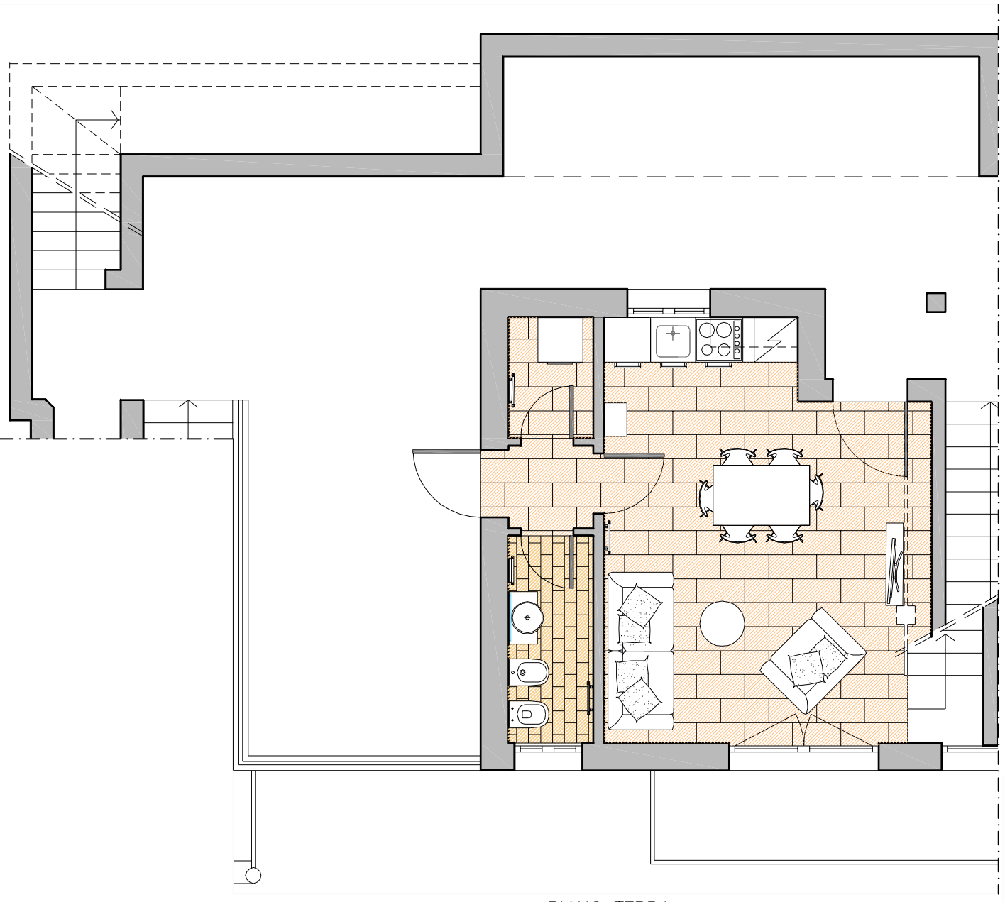
PIANO TERRA
